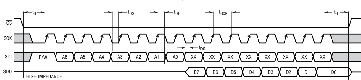
SPI Port Timing (Readback Mode)
