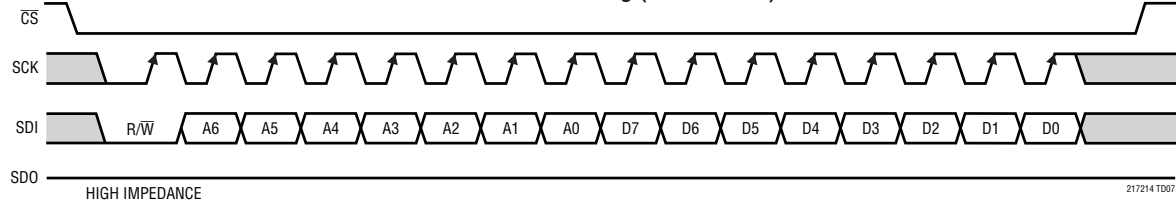
SPI Port Timing (Write Mode)
